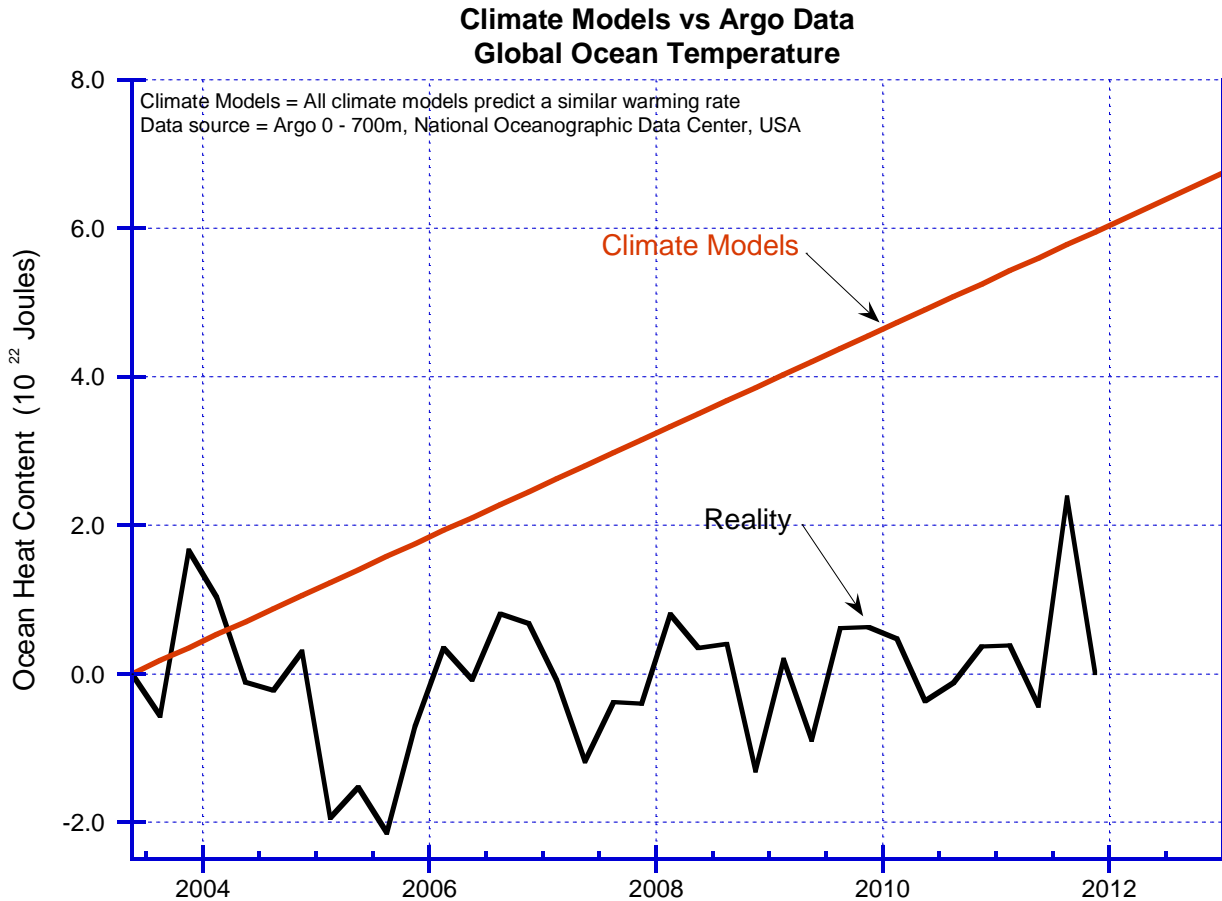
Figure 5: Climate model predictions 11 of ocean temperature, versus the measurements by Argo 12 . The unit of the vertical axis is 10 22 Joules (about 0.01°C).
