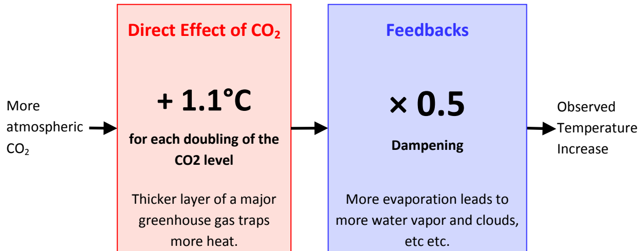
Figure 2: The sceptic's view. If the CO 2 level doubles, sceptics estimates that the temperature increase due to that extra CO 2 will be about 1.1^{\circ}\text{C} \times 0.5 \approx 0.6^{\circ}\text{C} . 4
