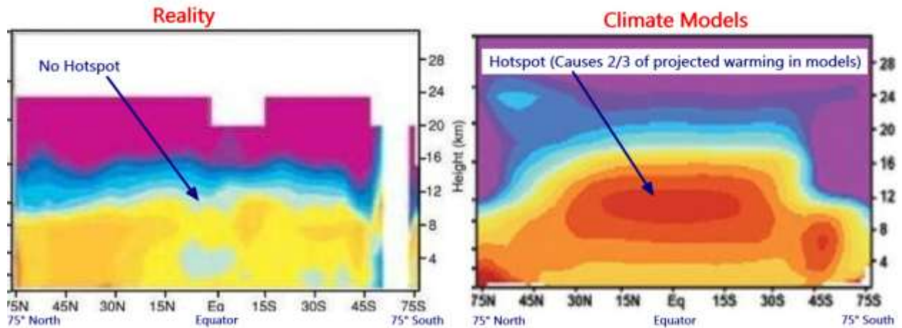
Figure 6: On the left is the data collected by millions of weather balloons. 14 On the right is what the climate models say was happening. 15 The theory (as per the climate models) is incompatible with the observations. In both diagrams the horizontal axis shows latitude, and the right vertical axis shows height in kilometers.
