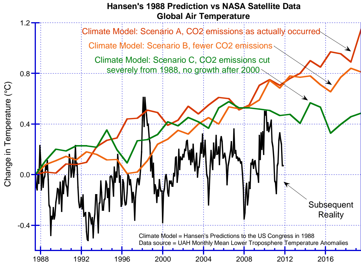
Figure 3: Hansen's predictions 6 to the US Congress in 1988, compared to the subsequent temperatures as measured by NASA satellites 7 .
